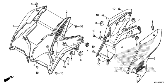
SIDE COVER
