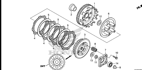
CLUTCH(1)(CHONGQING WANG CHENG)
