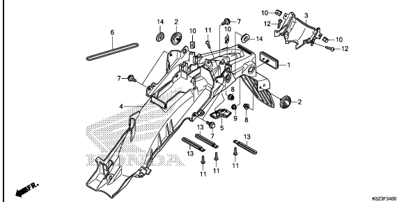
REAR FENDER
