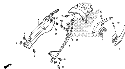
REAR COWL
