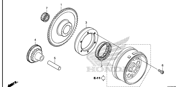
STARTING CLUTCH
