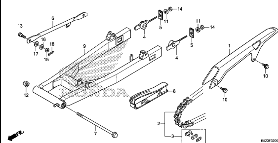
SWINGARM
