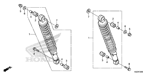
REAR CUSHION
